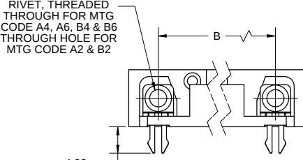
RIGHT ANGLE PLASTIC BRACKET WITH BOARD LOCK
