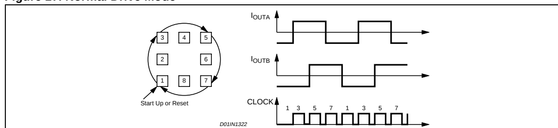
Figure 17. Normal Drive Mode
