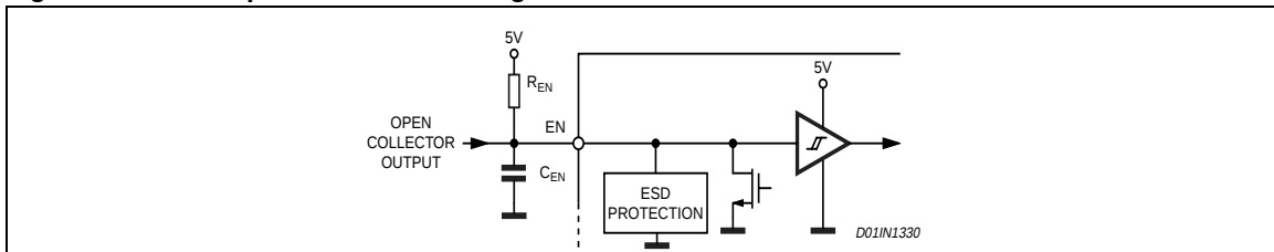
Figure 8. EN Pin Open Collector Driving
