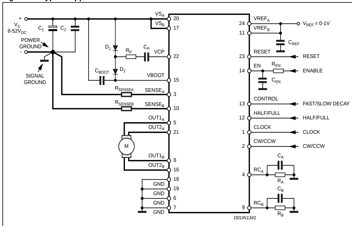
Figure 23. Typical Application
