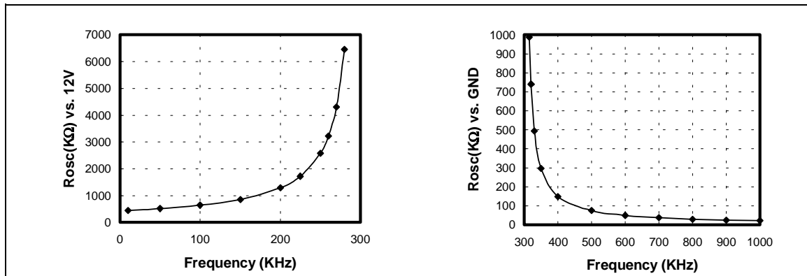
Figure 1. R_{\text{OSC}} vs. Switching Frequency
