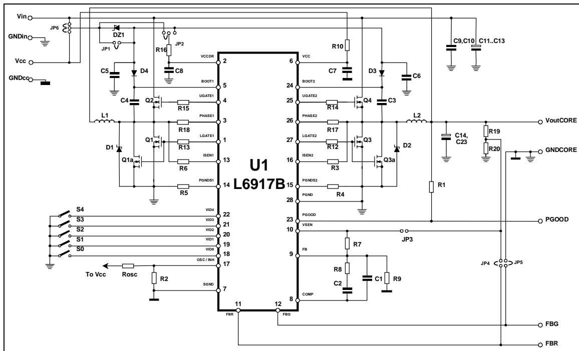
Figure 27. Server power supply schematic
