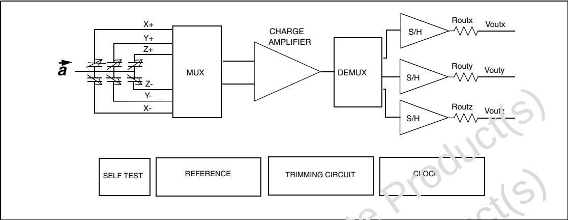
Figure 1. Block Diagram
