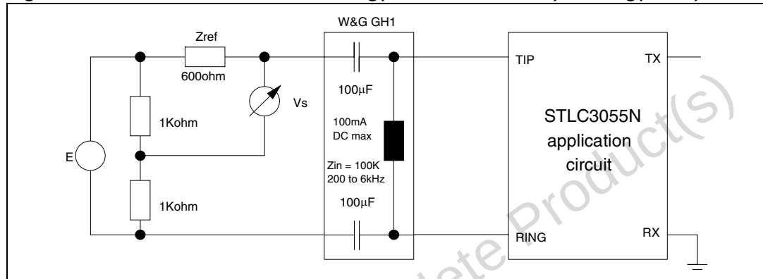
Figure 11. THL trans hybrid loss THL = 20\text{Log}|V_{\text{rx}}/V_{\text{tx}}|
