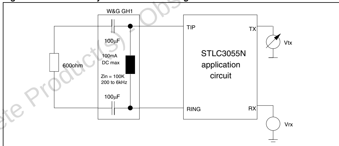
Figure 11. THL trans hybrid loss THL = 20\text{Log}|V_{\text{rx}}/V_{\text{tx}}|
