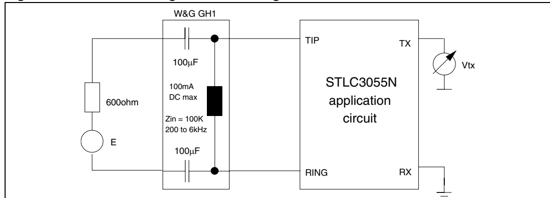
Figure 12. G24 transmit gain G24 = 20\text{Log}|2V_{\text{tx}}/E|
