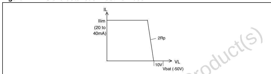
Figure 4. DC characteristic in active mode
