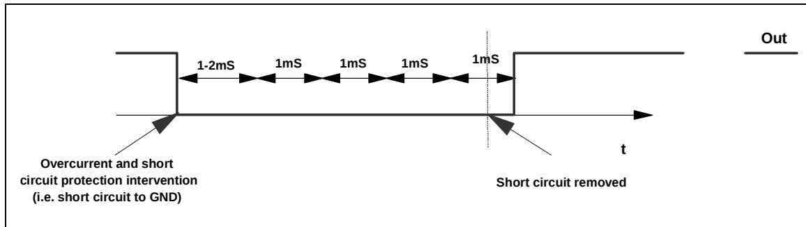
Figure 15. Restart timing with Diagnostic Enable
