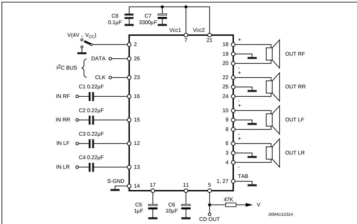
Figure 1. Application Circuit
