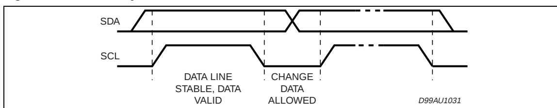
Figure 17. Timing Diagram on the I 2 C BUS
