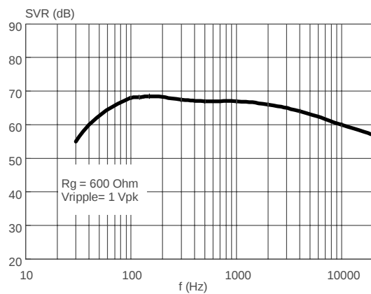
Figure 10. Supply Voltage Rejection vs. Freq.
