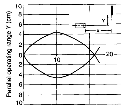
E3S-BD□1 (Left and Right)
