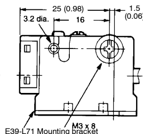
E39-L71 Mounting bracket
