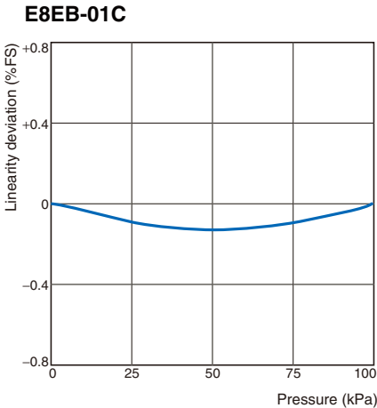
Linearity E8EB-01C
