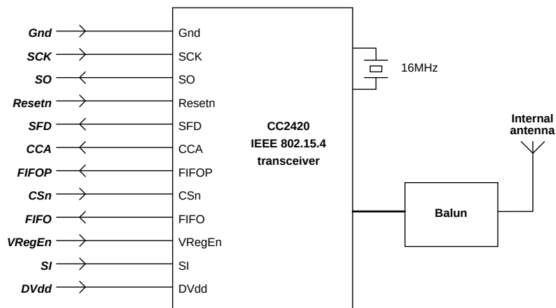
Figure 2. EasyBee Functional Block Diagram
