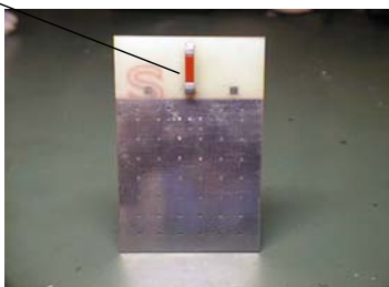
Helical Chip Antenna Top Side
