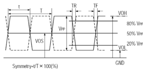
Figure 4) Output Waveform
