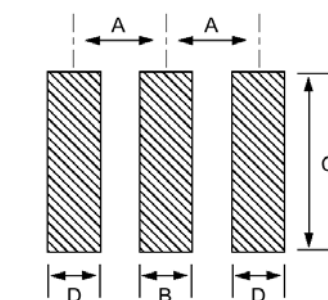
Figure 2) Land Pattern
