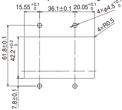
Multiple Mounting
