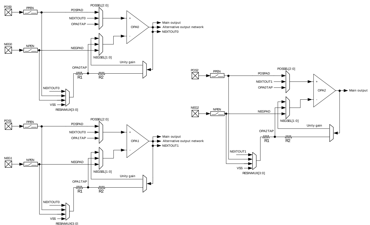
Figure 30.2. OPAMP Overview
