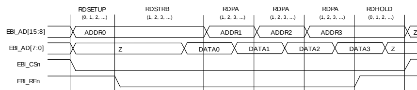
Figure 14.12. EBI Page Mode Read Operation for D16A16ALE addressing mode
