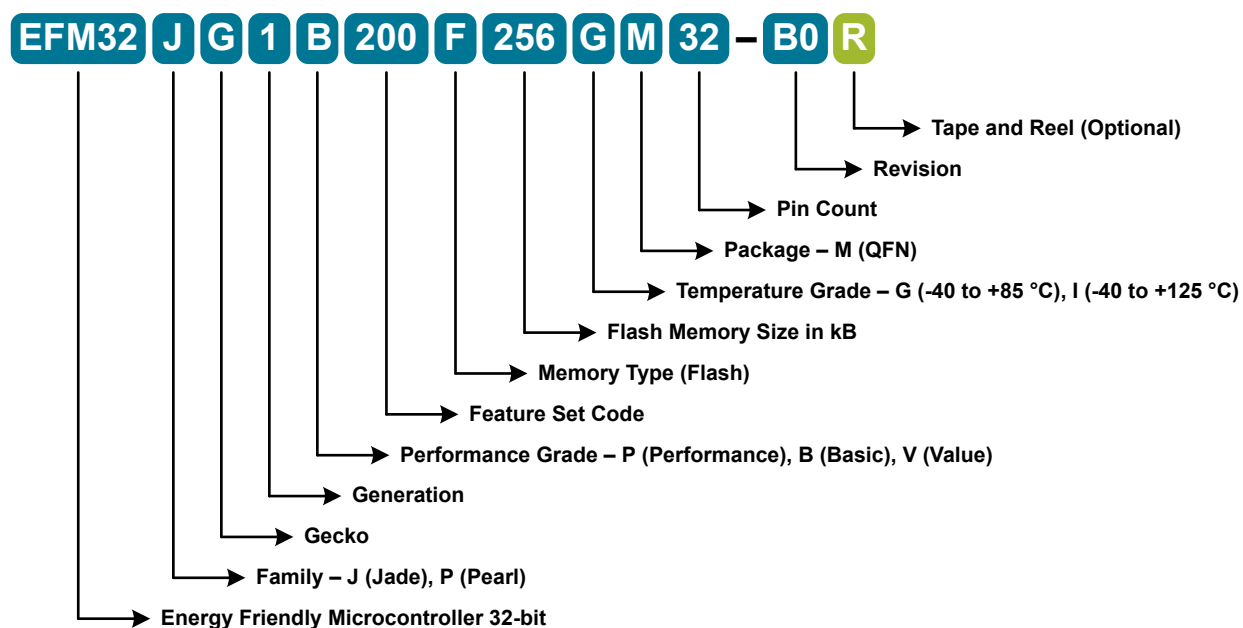
Figure 2.1. OPN Decoder
