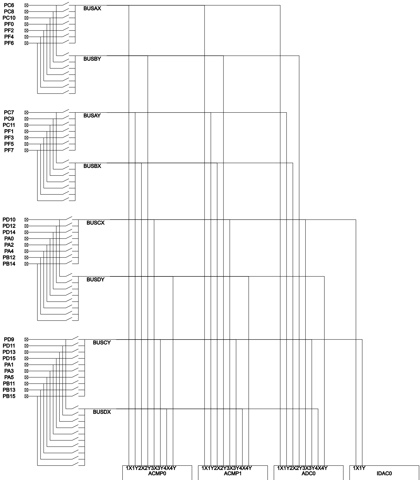
Figure 6.4. EFM32JG1 APORT
