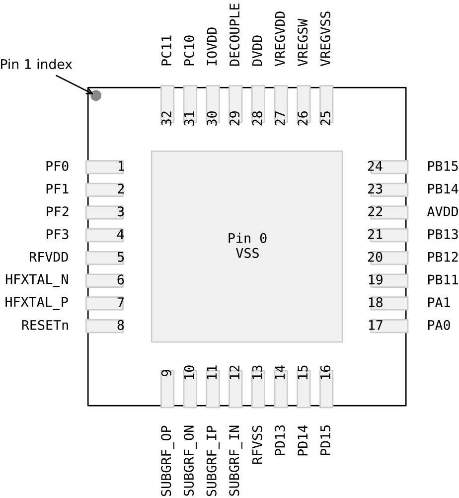
Figure 6.5. EFR32FG1 QFN32 Sub-GHz Pinout
