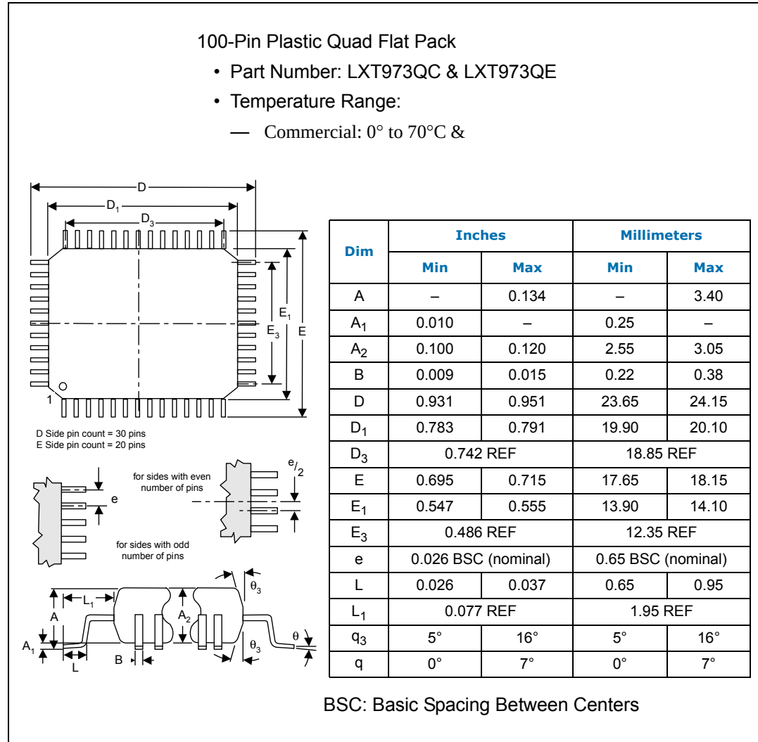
Figure 43 Mechanical Specifications
