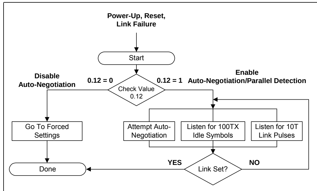
Figure 8 Auto-Negotiation Operation
