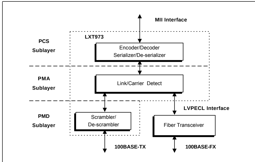
Figure 10 Protocol Sublayers
