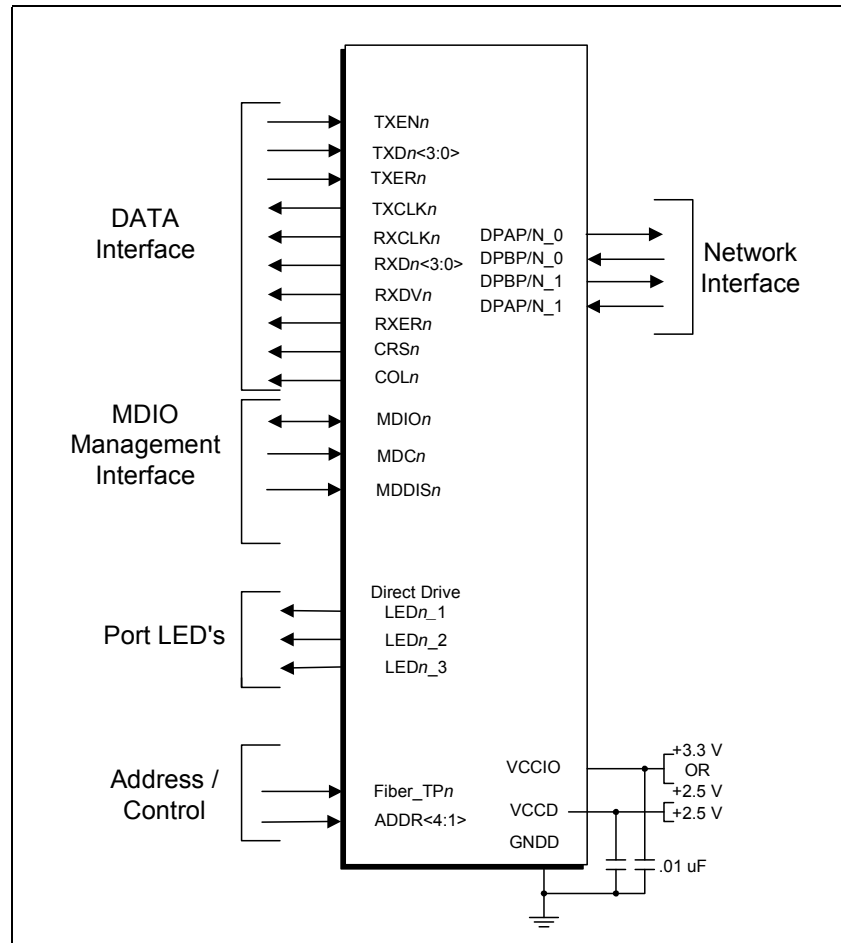
Figure 3 Interfaces
