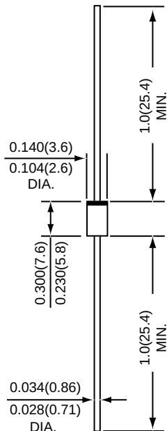
DO-204AC
