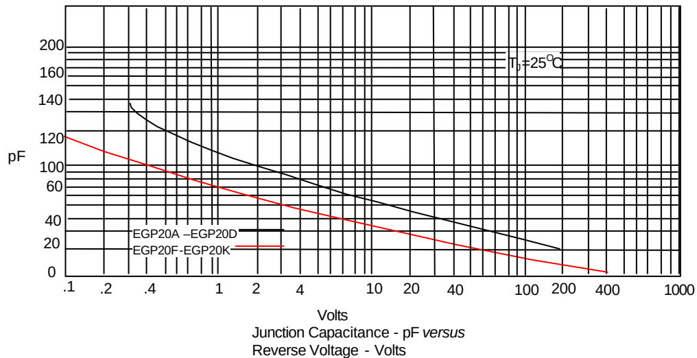
Figure 3 Junction Capacitance
