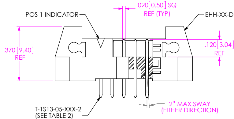
FIG 1 (EHT-105-01-XX-D SHOWN) (LATCH EHA-01 REMOVED FOR CLARITY)
