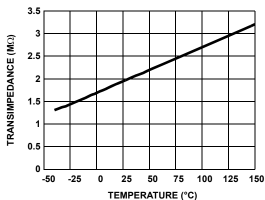
FIGURE 48. TRANSIMPEDANCE vs TEMPERATURE
