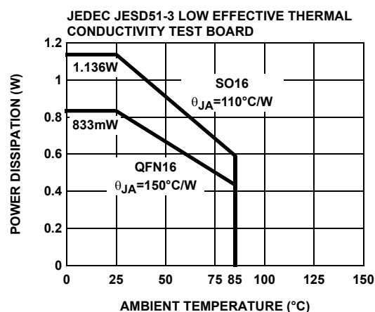
FIGURE 49. PACKAGE POWER DISSIPATION vs AMBIENT TEMPERATURE
