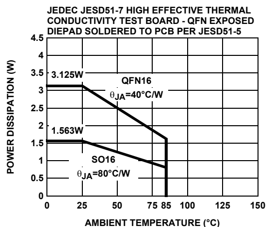
FIGURE 50. PACKAGE POWER DISSIPATION vs AMBIENT TEMPERATURE
