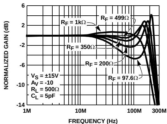
FIGURE 4. INVERTING FREQUENCY RESPONSE FOR VARIOUS R_F
