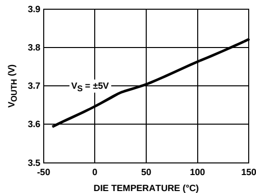
FIGURE 40. POSITIVE OUTPUT SWING vs TEMPERATURE
