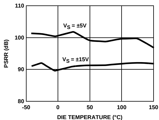
FIGURE 38. PSRR vs TEMPERATURE
