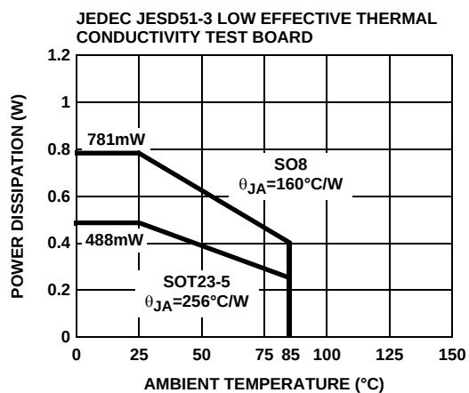
FIGURE 48. PACKAGE POWER DISSIPATION vs AMBIENT TEMPERATURE
