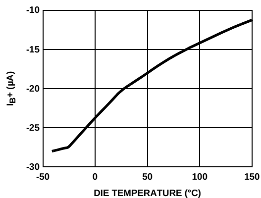
FIGURE 36. INPUT BIAS CURRENT vs TEMPERATURE
