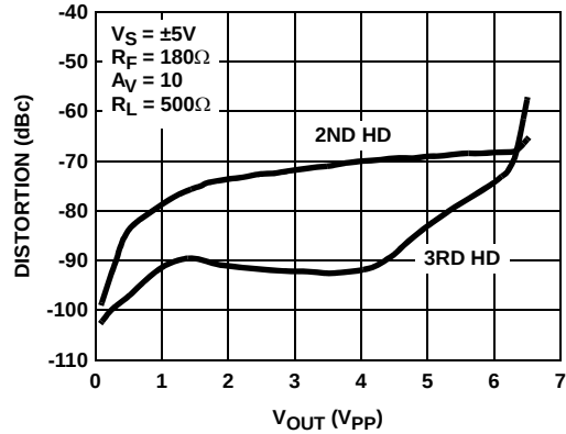
FIGURE 23. 1MHz HARMONIC DISTORTION vs OUTPUT SWING
