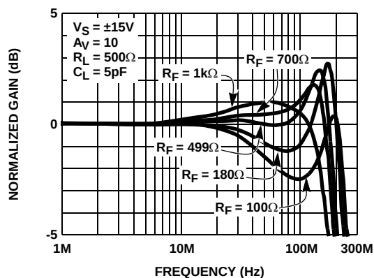
FIGURE 2. NON-INVERTING FREQUENCY RESPONSE FOR VARIOUS R_F
