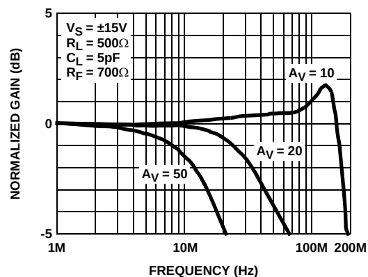
FIGURE 6. NON-INVERTING FREQUENCY RESPONSE FOR VARIOUS GAIN
