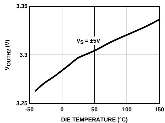
FIGURE 46. LOADED POSITIVE OUTPUT SWING vs TEMPERATURE
