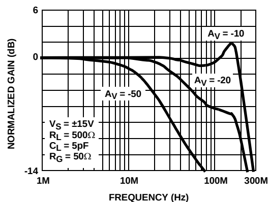
FIGURE 8. INVERTING FREQUENCY RESPONSE vs GAIN
