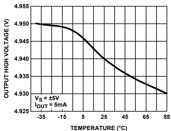
FIGURE 12. OUTPUT HIGH VOLTAGE vs TEMPERATURE
