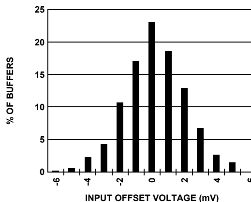
FIGURE 10. INPUT OFFSET VOLTAGE DISTRIBUTION
