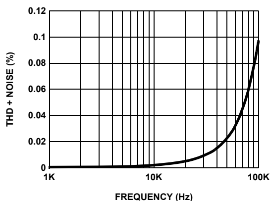
FIGURE 6. TOTAL HARMONIC DISTORTION + NOISE vs FREQUENCY
