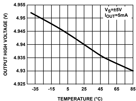
FIGURE 10. OUTPUT HIGH VOLTAGE vs TEMPERATURE
