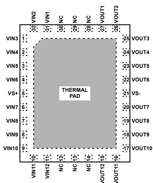
EL5427 (32 LD QFN) TOP VIEW
