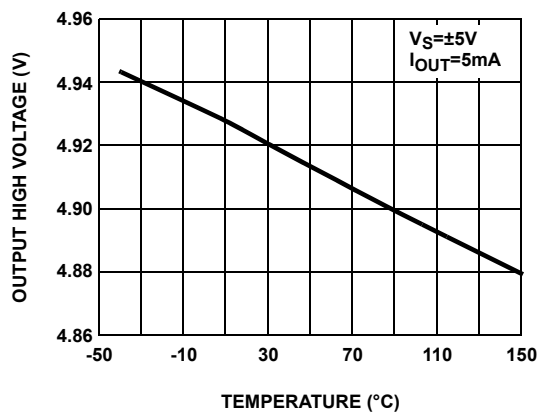
FIGURE 5. OUTPUT HIGH VOLTAGE vs TEMPERATURE
