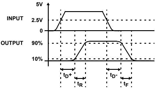
Timing Diagram
