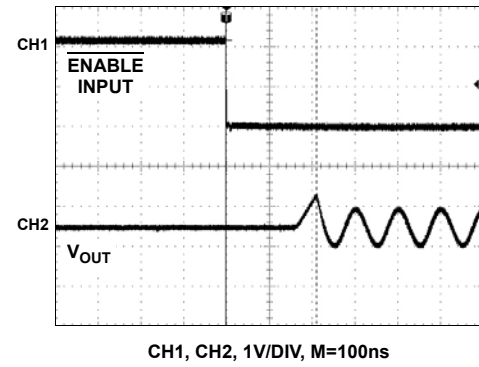
FIGURE 26. ENABLED RESPONSES
