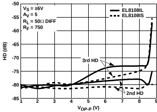
FIGURE 9. DISTORTION BETWEEN EL8108IL vs EL8108IS AT 2MHz
