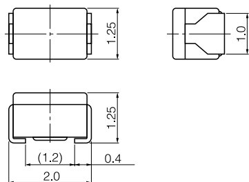
Type ND (2.0×1.25×1.25)
