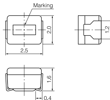
Types FC, NC, PC (2.5×2.0×1.6)
