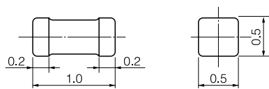
Type RF (1.0×0.5×0.5)
