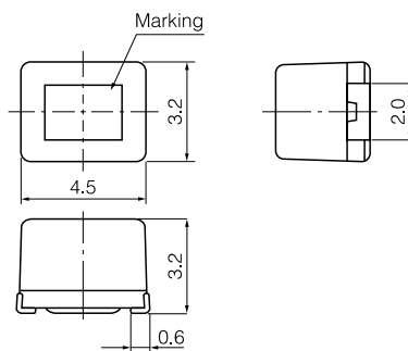
Type FB (4.5×3.2×3.2)
