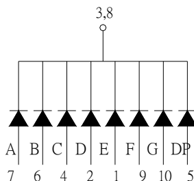
Internal Connection Diagram
