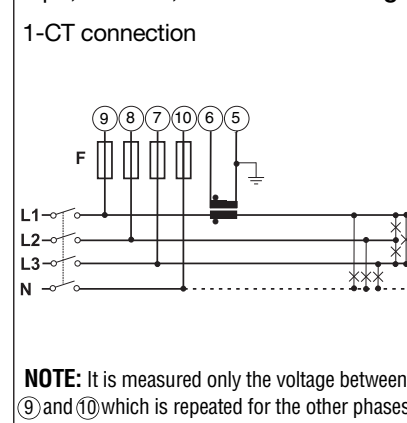
3-ph, 3/4-wire, balanced load Fig. 7
