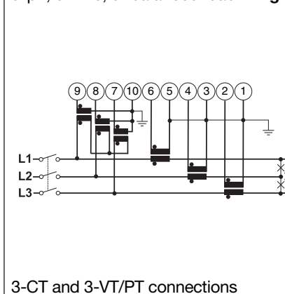
3-ph, 3-wire, unbalanced load Fig. 4
