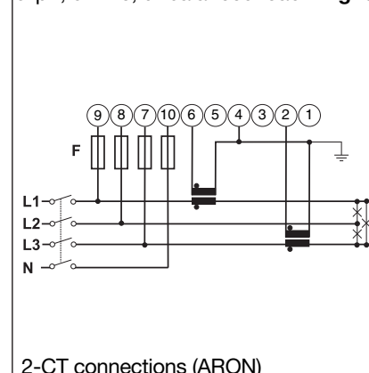
3-ph, 3-wire, unbalanced load Fig. 5
