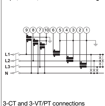
3-ph, 4-wire, unbalanced load Fig. 2
