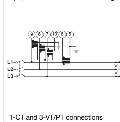
3-ph, 3-wire, balanced load Fig. 8
