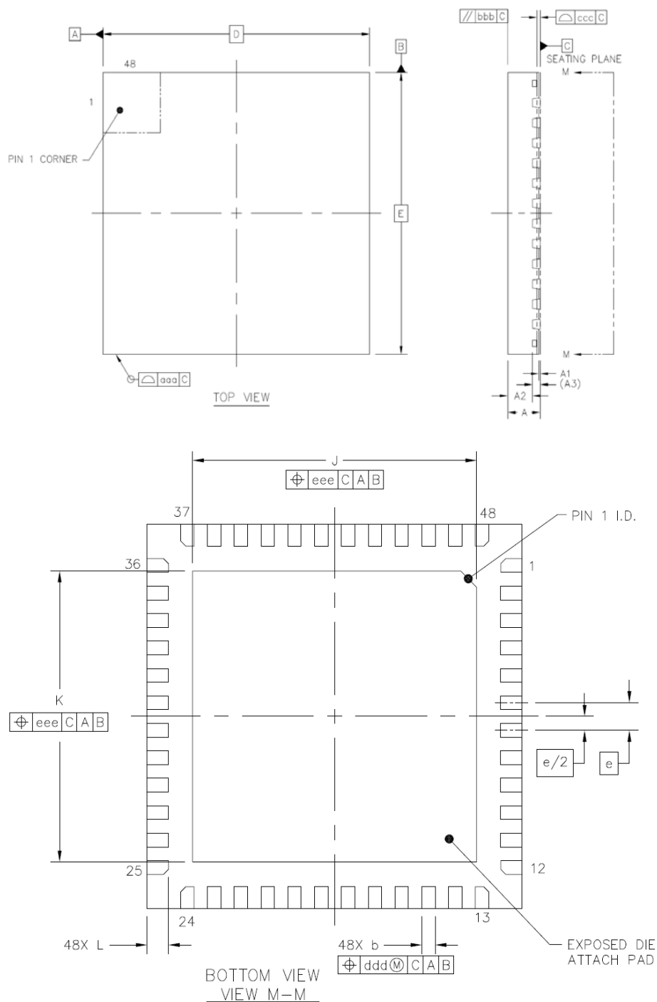
Figure 6.2. Package Drawing
