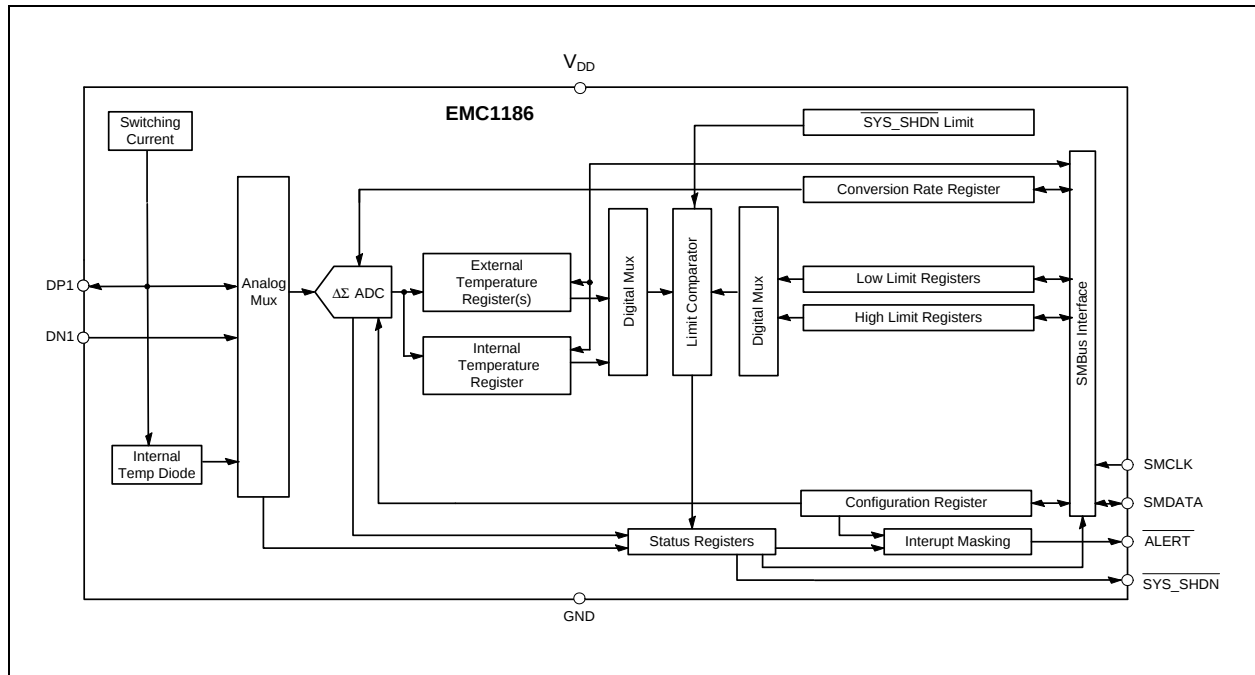
Figure 1.1 EMC1186 Block Diagram
