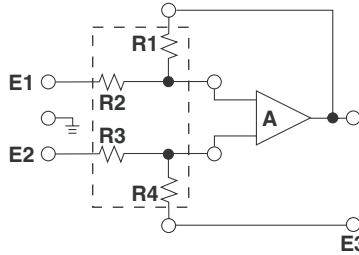
FIGURE 4 - VISHAY MODEL 300198 NETWORK
