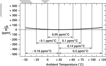
FIGURE 2 - TYPICAL TCR CURVE Z-FOIL
