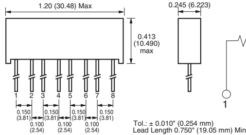
FIGURE 7 - MOLDED 2R, 3R, 4R RESISTOR NETWORK DIMENSIONS AND CIRCUIT DESIGN in inches (millimeters)
