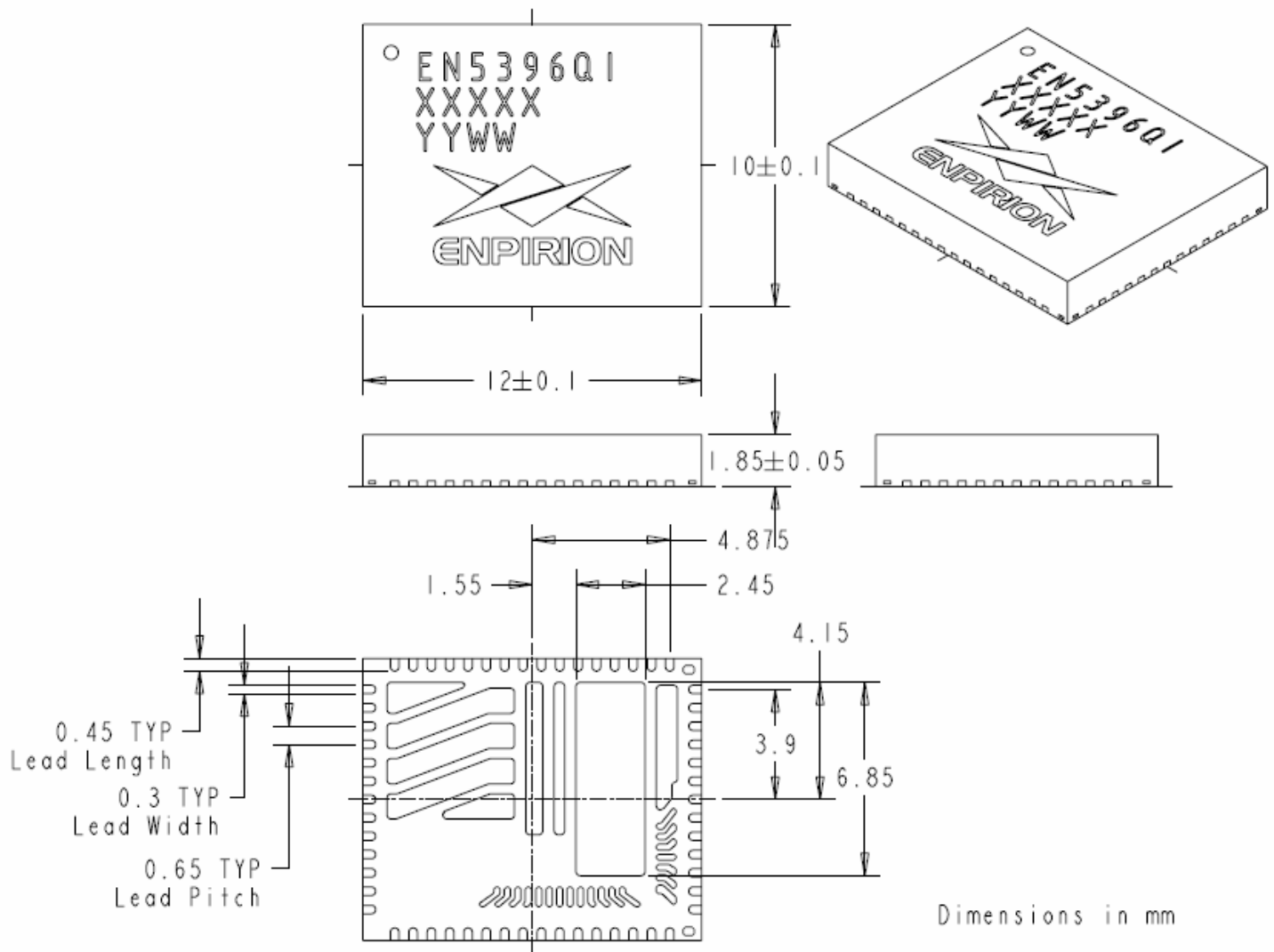
Figure 11. Package dimensions.
