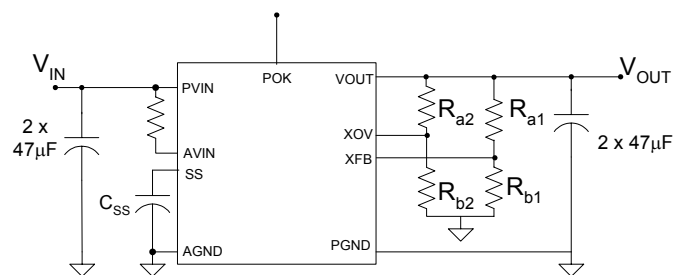
Figure 4. V_{OUT} and OVP resistor divider networks.
