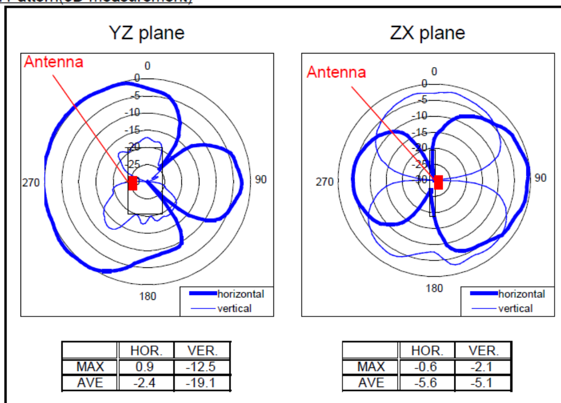
Fig. 5 Condition 1: LDA21K
