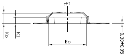
SECTION Y-Y
