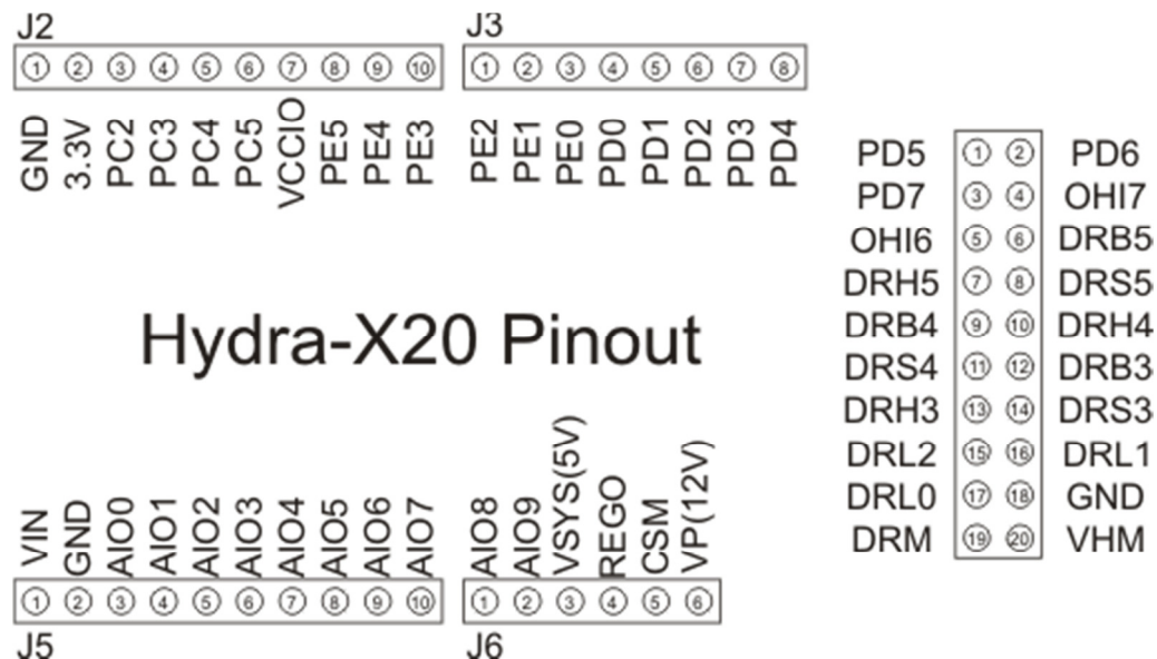
Figure 2 HYDRA-X20 Pinout
