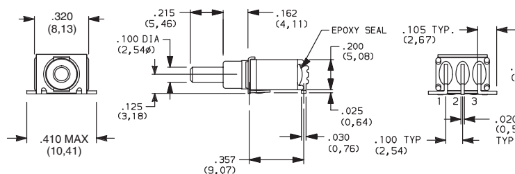
EP12SD1SAPE SPDT
