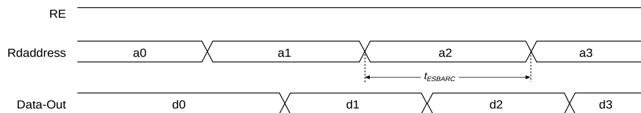
Figure 38. ESB Asynchronous Timing Waveforms
