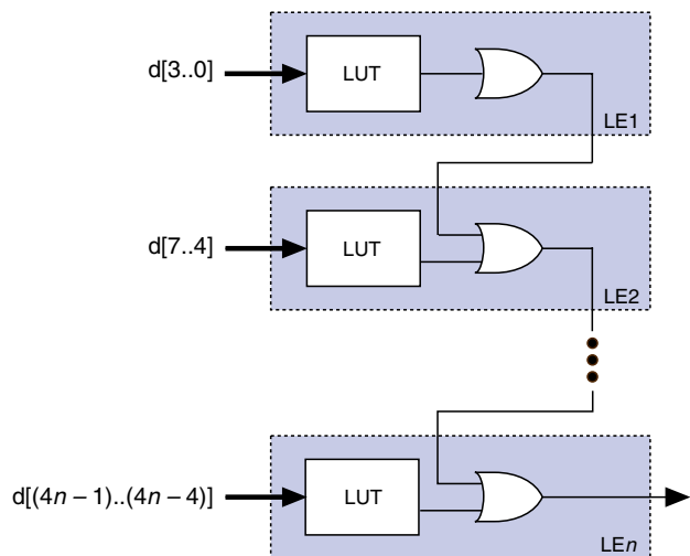
OR Cascade Chain
