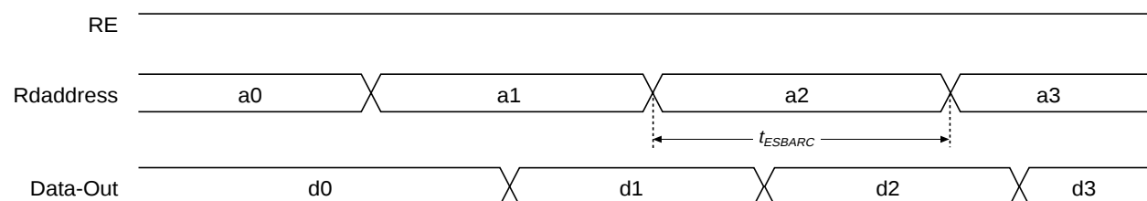
Figure 38. ESB Asynchronous Timing Waveforms
