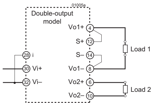
Fig. 5 Independent-output configuration
