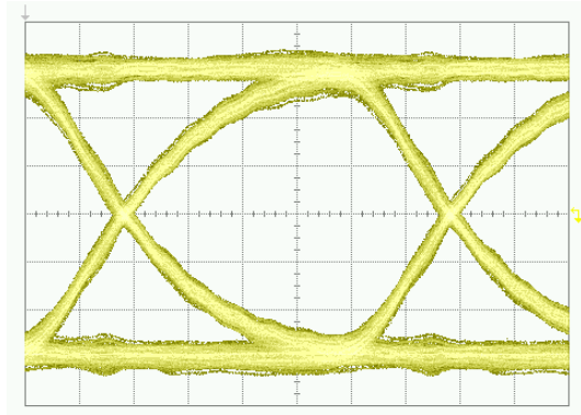
2m CAT6 cable before equalizer
