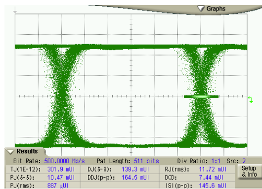
300mV Transmit amplitude (80m CAT6 cable)
