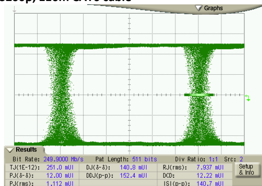
S200β, 110m CAT6 cable
