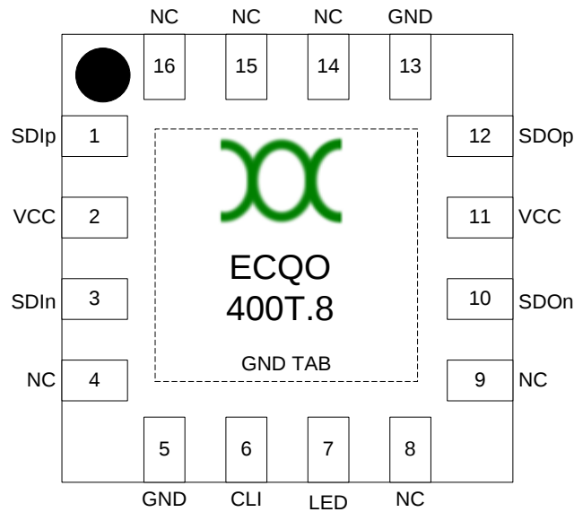
Figure 3: EQCO400T8 Pin Layout (viewed from top)
