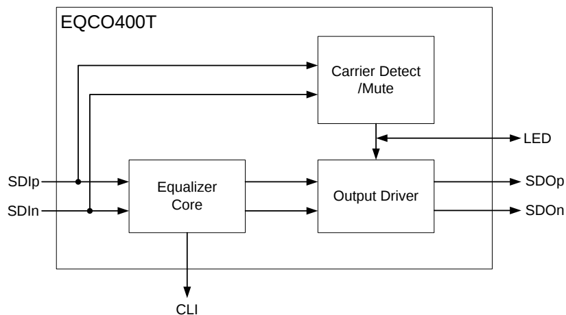
Figure 2: EQCO400T8 block diagram showing electrical connections
