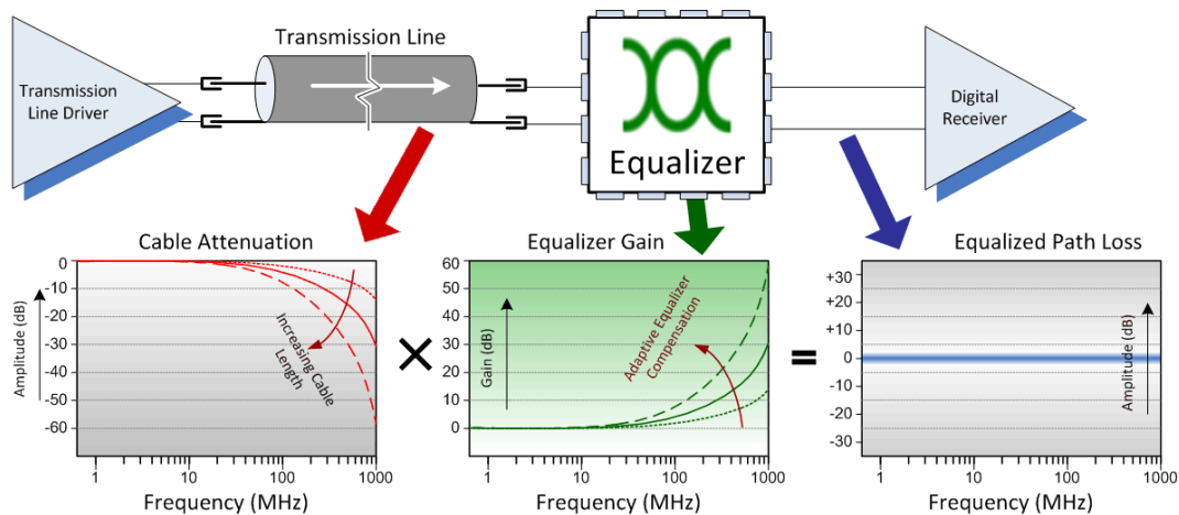
Figure 5: Principle of Equalizer Operation
