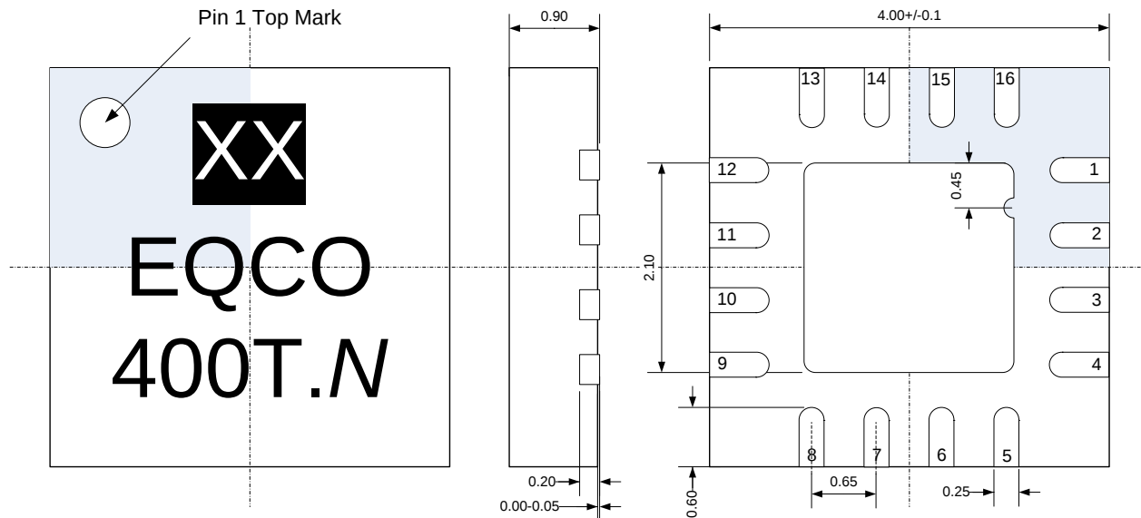
Figure 6: Package Drawing viewed from Top - Side - Bottom 4
