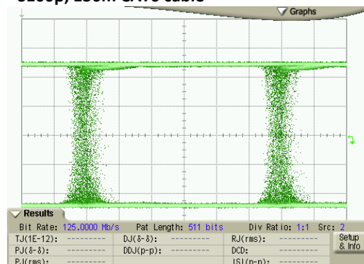
S100β, 130m CAT6 cable
