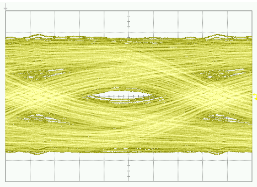
30m CAT6 cable before equaliser
