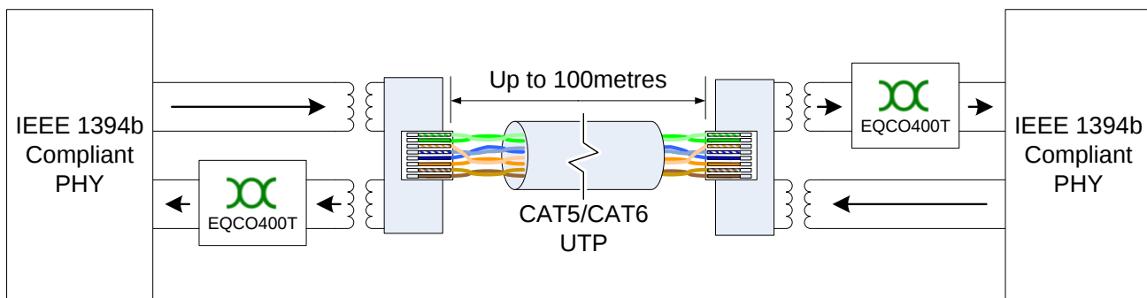
Figure 1: Long-haul IEEE 1394b-2002, IEEE 1394-2008 connection
