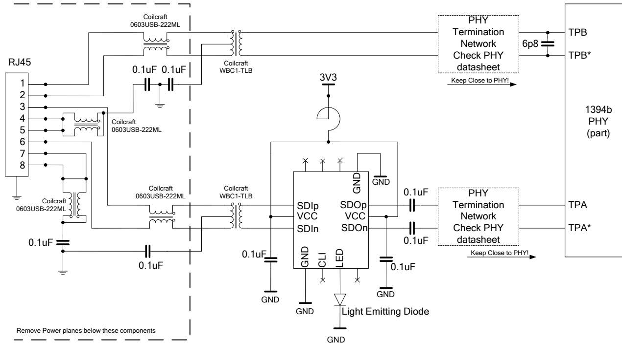
Figure 8: Example Schematic Implementation
