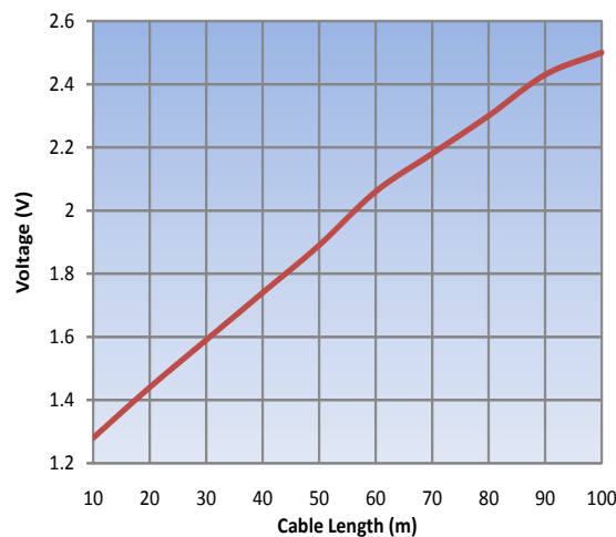
Figure 4: CLI voltage as a function of cable length (Systimax CAT6 cable)
