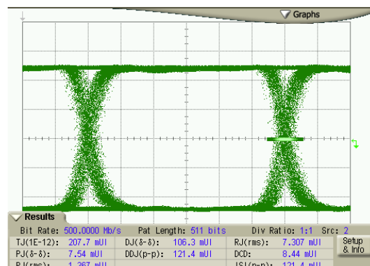
800mV Transmit amplitude (80m CAT6 cable)
