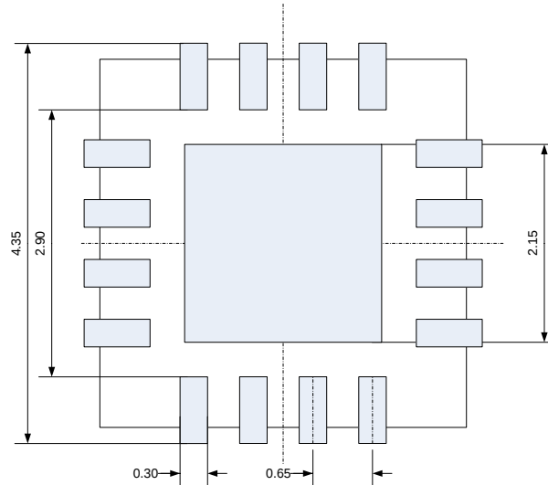
Figure 7: Recommended PCB Footprint
