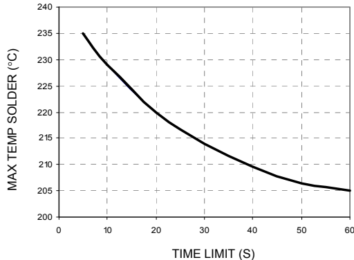
Figure 50. Time Limit, T lim , Curve Above 205°C Reflow .
