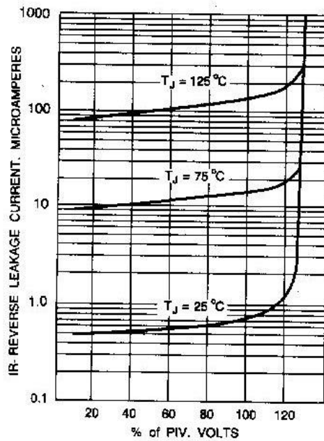
Fig. 3-TYPICAL REVERSE CHARACTERISTICS
