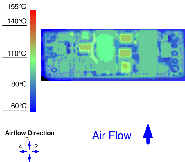
Figure 12. Thermal Image for Airflow Direction 3 (25A output, 55 ^{\circ}C ambient, 200 LFM, V_{in} = 48V open frame unit using socket interface)
