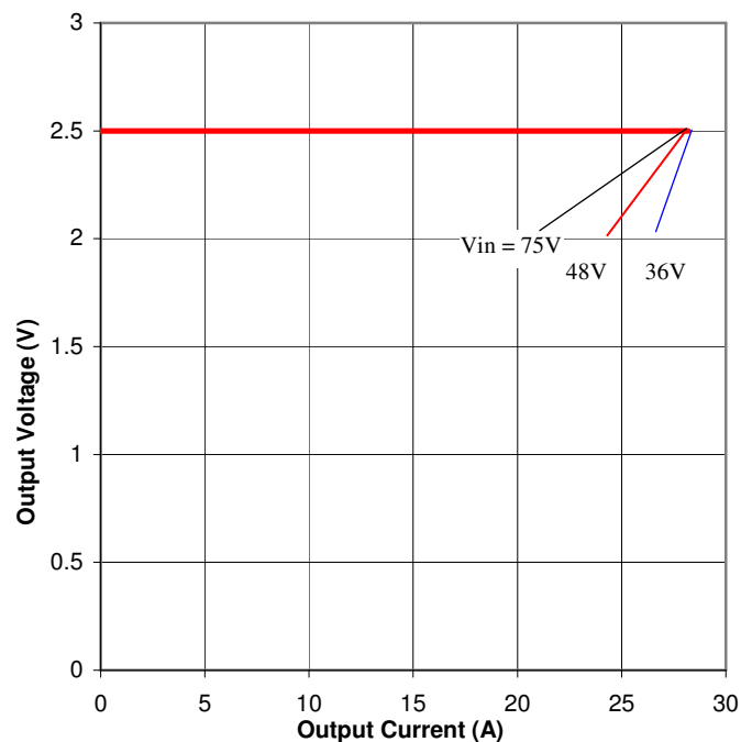
Figure 10. Output Characteristics
