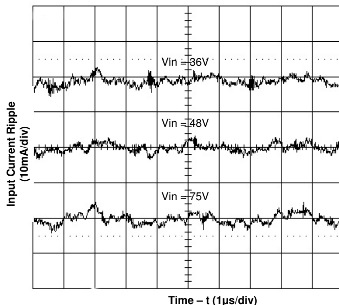
Figure 6. Input Reflected Ripple Current at 25A Load
