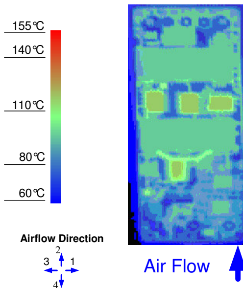
Figure 14. Thermal Image for Airflow Direction 2 (23.2A output, 55°C ambient, 200 LFM, Vin = 48V open frame unit using solder interface)
