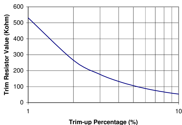
Fig. 19 Trim-Up Resistor Selection
