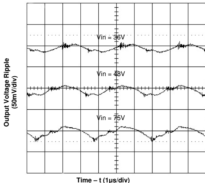
Figure 5. Output Ripple Voltage at 25A Load
