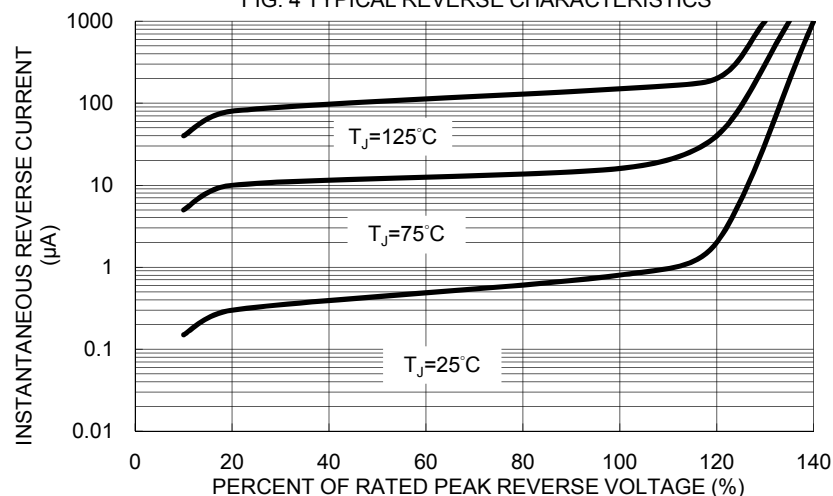
FIG. 4 TYPICAL REVERSE CHARACTERISTICS
