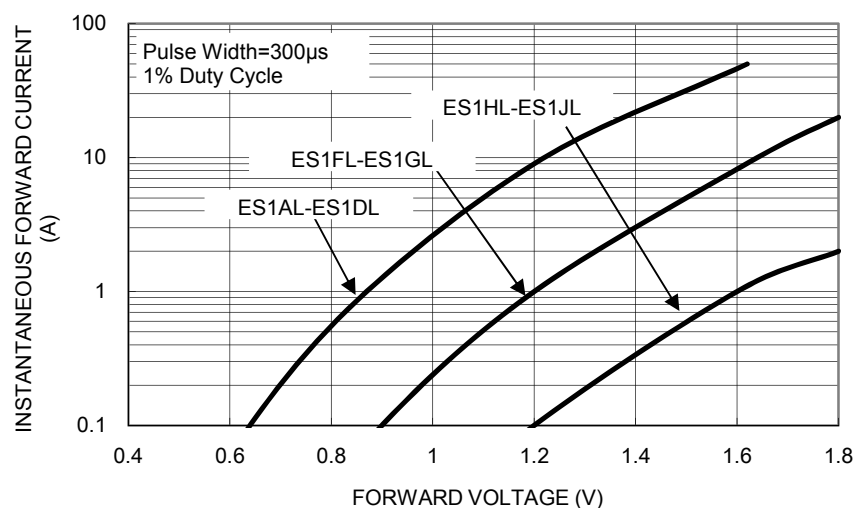
FIG. 2 TYPICAL FORWARD CHARACTERISTICS
