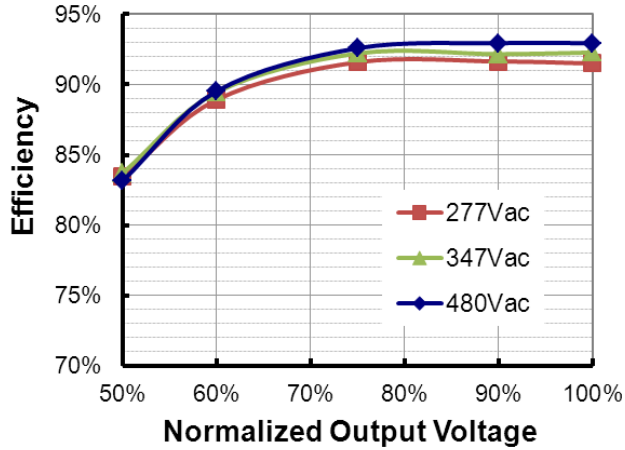
ESD-240S460DT (Io=3220mA) Efficiency vs. Output Voltage
