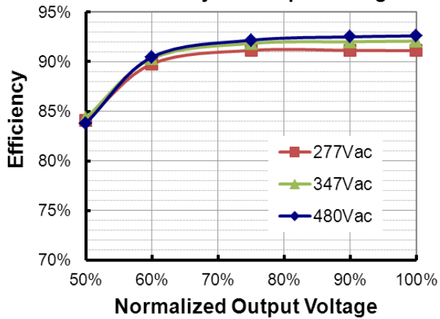
ESD-240S660DT (Io=4620mA) Efficiency vs. Output Voltage
