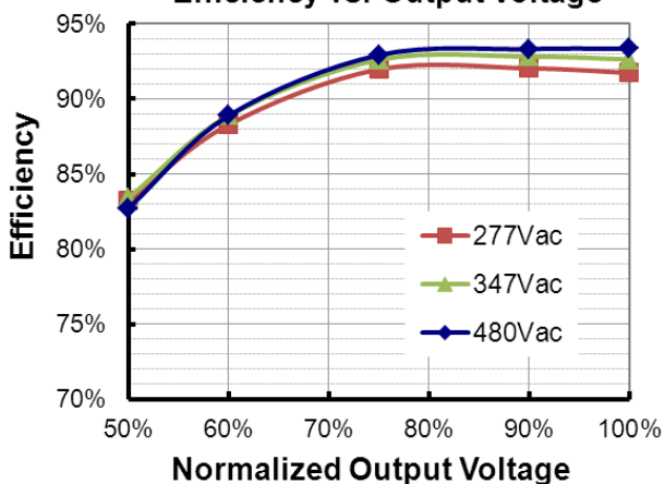
ESD-240S220DT( I_o=1540\text{mA} ) Efficiency vs. Output Voltage
