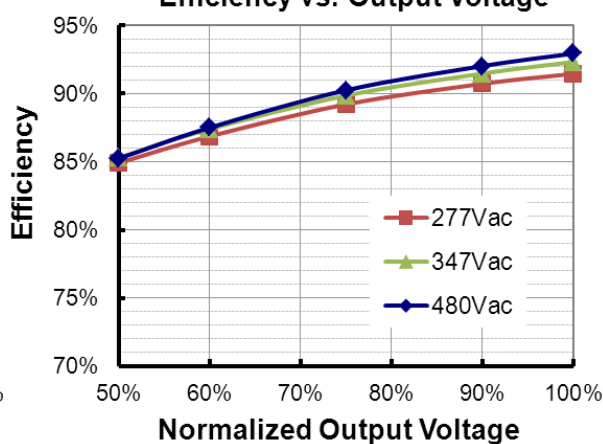
ESD-240S220DT( I_o=2200\text{mA} ) Efficiency vs. Output Voltage
