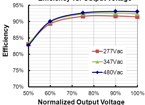
ESD-240S320DT( I_o=2240\text{mA} ) Efficiency vs. Output Voltage
