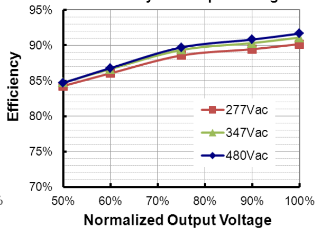
ESD-240S660DT (Io=6600mA) Efficiency vs. Output Voltage
