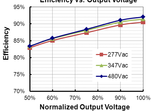
ESD-240S320DT( I_o=3200\text{mA} ) Efficiency vs. Output Voltage
