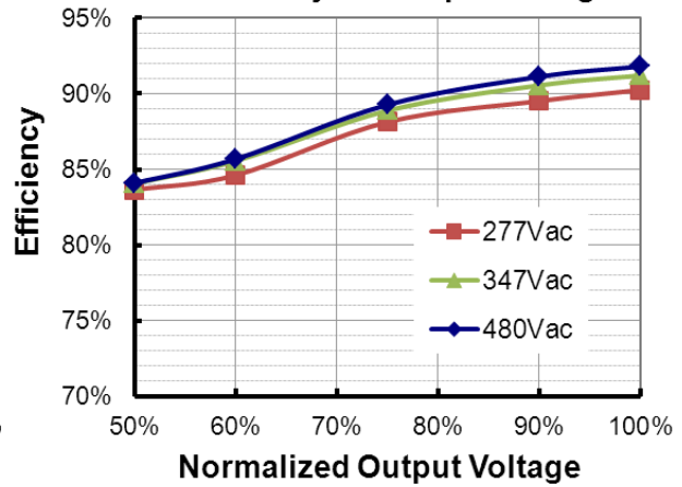
ESD-240S460DT (Io=4600mA) Efficiency vs. Output Voltage
