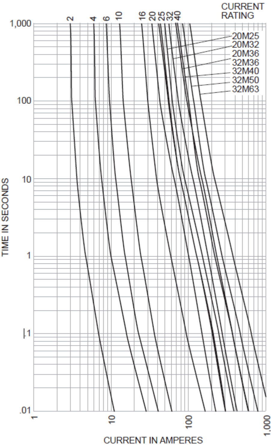
Time-Current Characteristic Curve (Full Size Curves Available)
