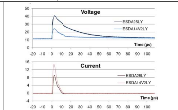
Figure 8. ISO 7637-2 pulse 2a response ( V_S = 50\text{ V} )
