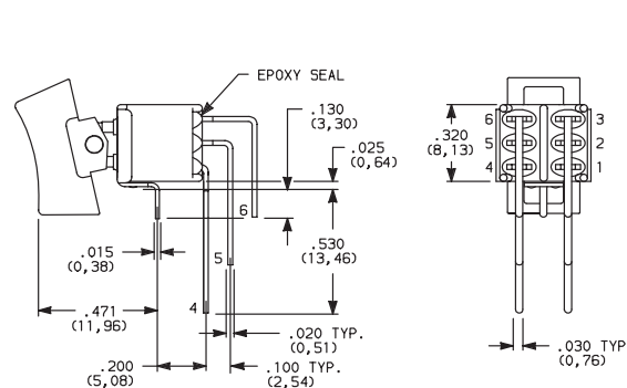
ET21J1AVBE2 Vertical Actuation DPDT Actuator Shown In Pos. 1
